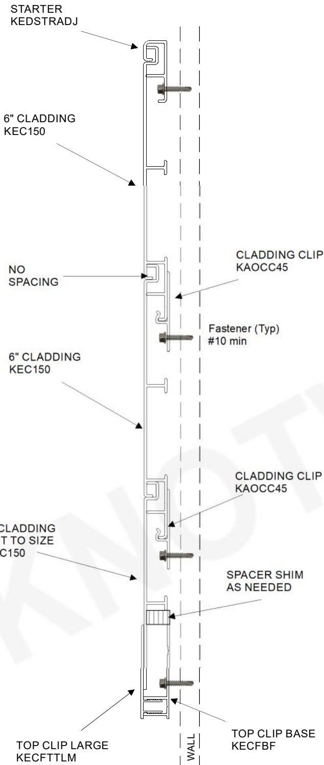
6" CLADDING TOP DOWN NO SPACING
