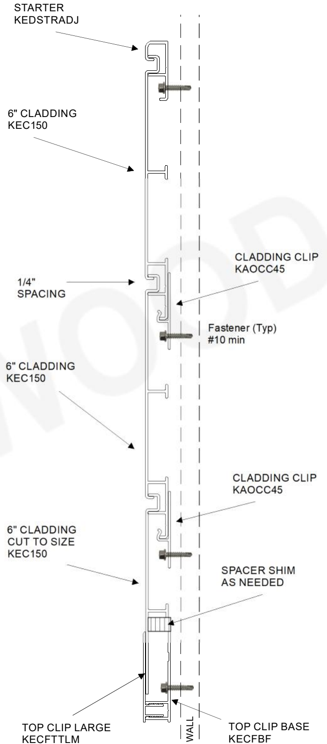
6" CLADDING TOP DOWN 1/4" SPACING
