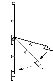
CLADDING CLIP
