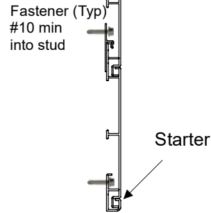
BOTTOM UP INSTALLATION
